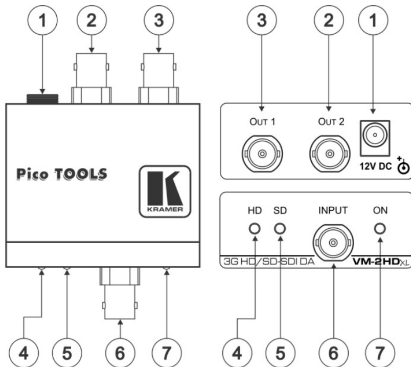
Figure 1: VM-2HDxl 3G HD/SD – SDI DA
