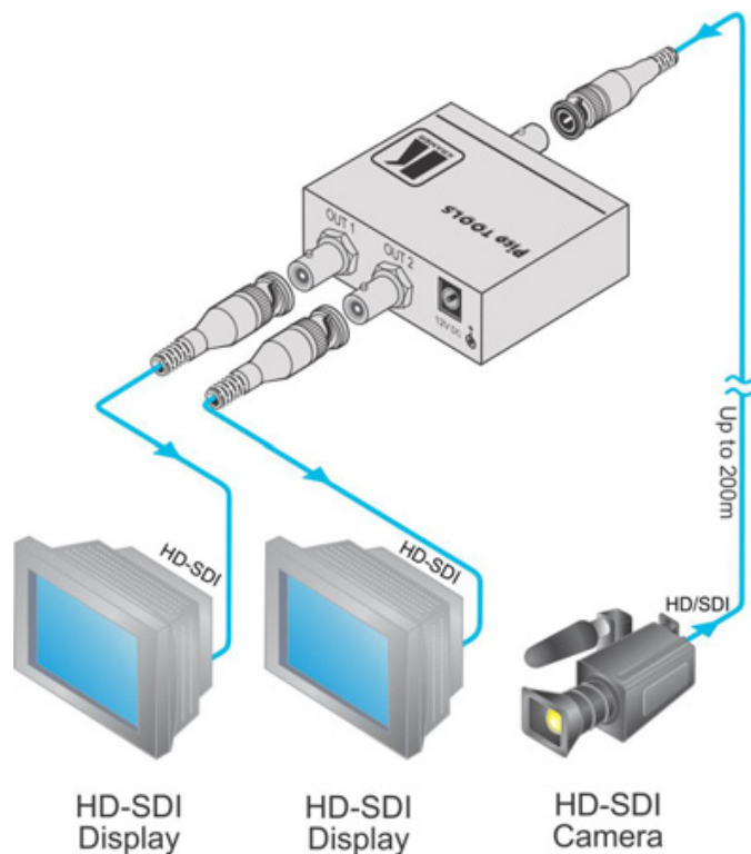
Figure 2: Connecting to the VM-2HDxI
