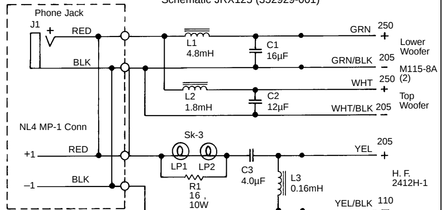
Schematic JRX125 (352929-001)
