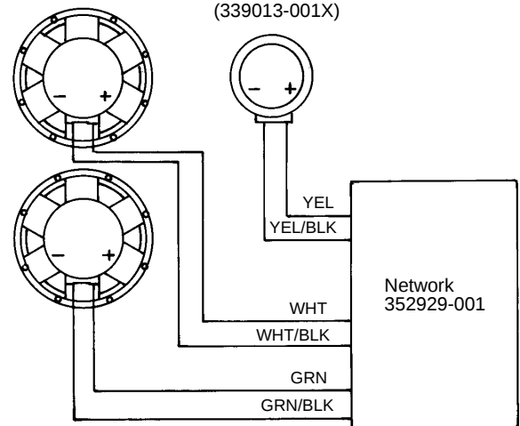
Schematic JRX125 (352929-001)
