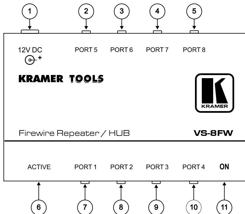
Figure 3: VS-8FW FireWire Repeater / HUB
