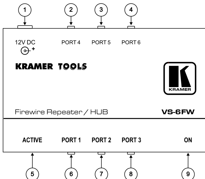
Figure 2: VS-6FW FireWire Repeater / HUB
