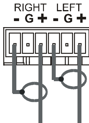
Figure 4: Connecting the Unbalanced Stereo Audio Input
