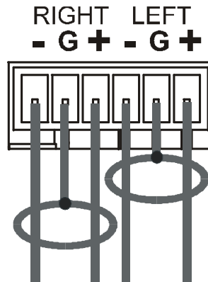
Figure 3: Connecting the Balanced Stereo Audio Input/Output
