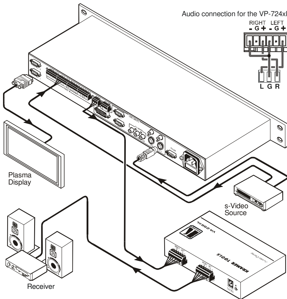
Figure 2: Connecting the VA-256xl Audio Delay
