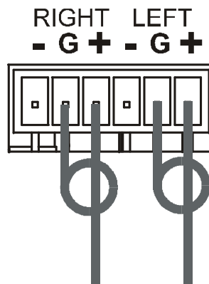
Figure 5: Connecting the Unbalanced Stereo Audio Output
