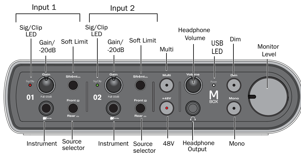
Figure 1. Mbox front panel
