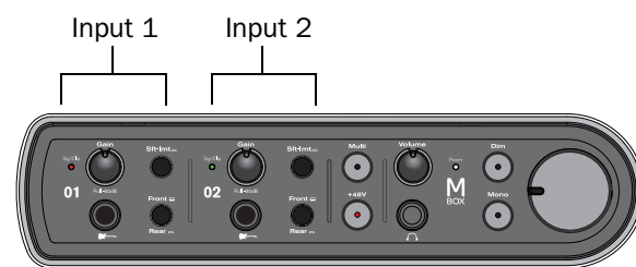
Inputs on front panel of Mbox
