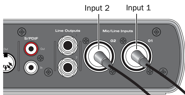
Mbox connections for line-level stereo input source
