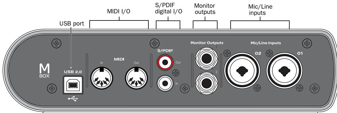
Figure 2. Mbox back panel
