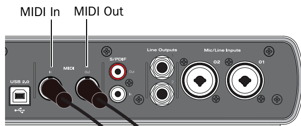
MIDI connections to Mbox
