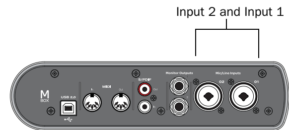
Inputs on rear panel of Mbox
