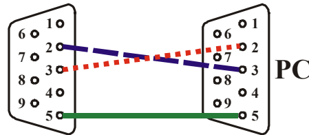
Figure 4: RS-232 Crossed Cable Connection
