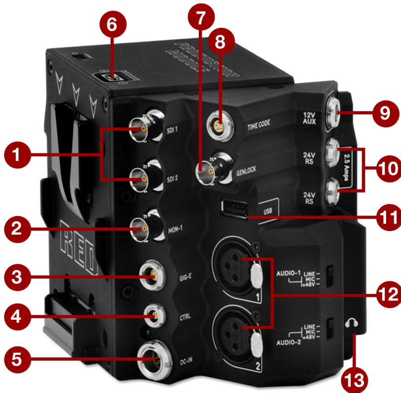
Figure: DSMC2 Production Module (V-Lock)
